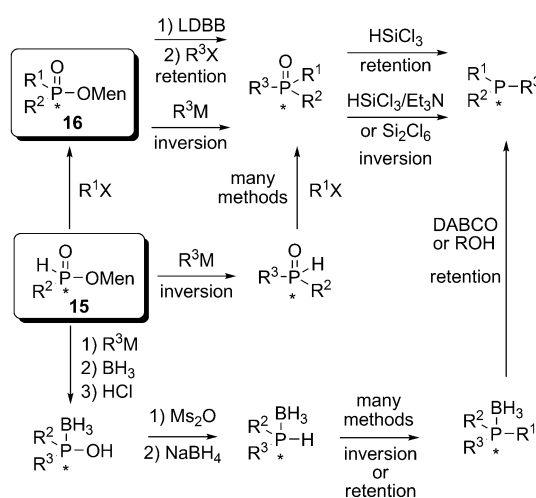
Scheme 6. Transformations of P-stereogenic menthyl phosphinates, described in the literature.
